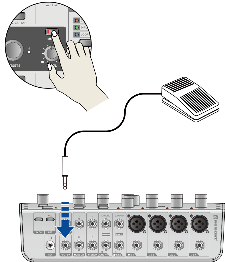
Connect to your pedal switch
